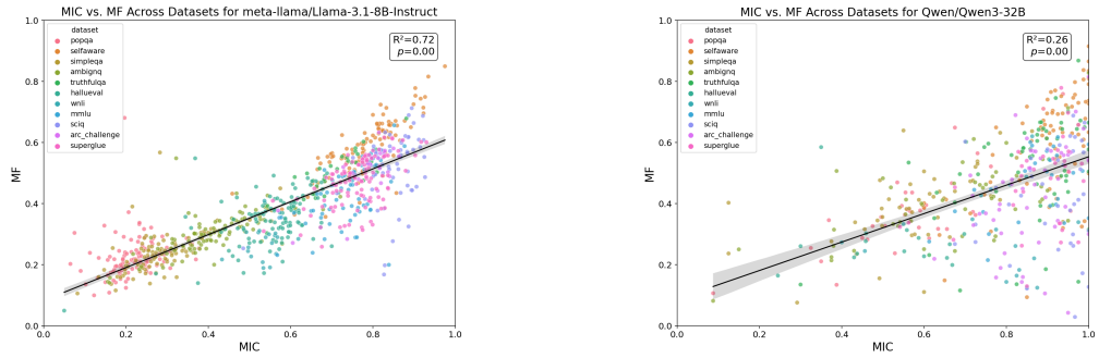
Figure 5: Representative plots of models' MICs in relation to per-marker average absolute difference between internal confidence and human-interpreted linguistic decisiveness (MF). We observe positive trends between internal confidence and human-model decisiveness divergence per marker, suggesting high-MIC markers are a primary driver of faithful miscalibration in LLMs when we interpret markers according to human perception.
