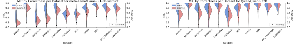
Figure 3: Representative violin plots of models' MIC densities across datasets, stratified by correctness. Dataset-level accuracy is indicated by black points (values along the second y -axis).
